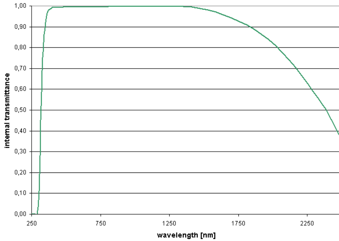
N-BK7 Transmittance (25 mm thickness)
